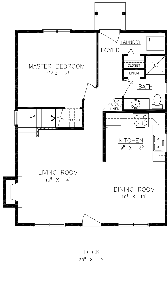
MAIN FLOOR AREA = 810 S.F.
