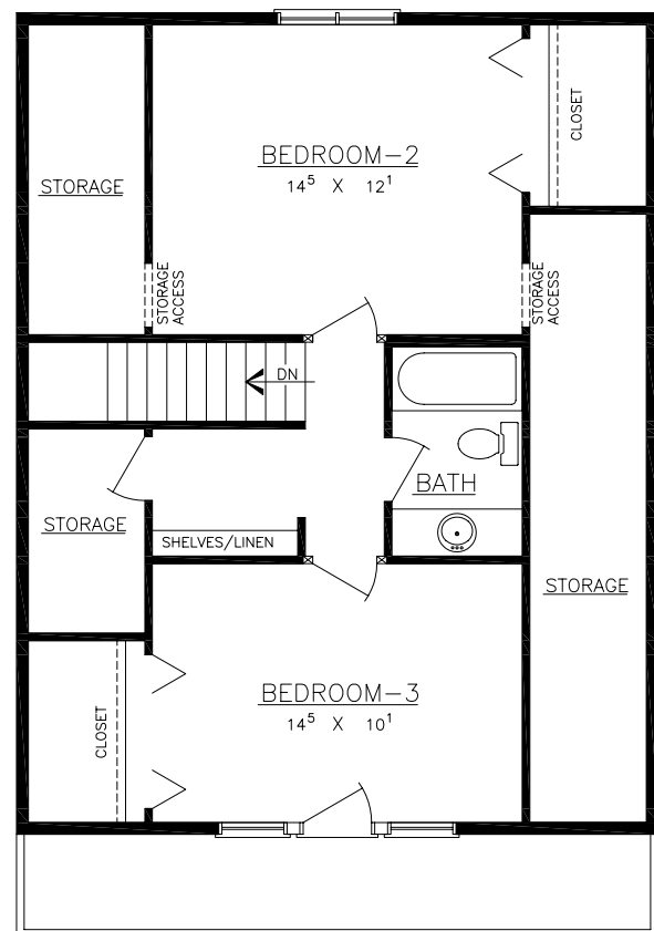
SECOND FLOOR AREA = 461 S.F.
